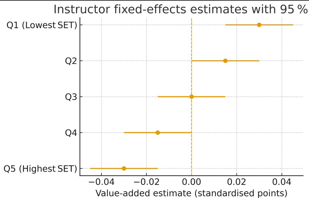
Figure 3. Instructor fixed-effects estimates (circles) with 95 % confidence intervals (horizontal bars) from hierarchical value-added models predicting follow-on student performance. Estimates for instructors in the highest student-evaluation-of-teaching (SET) quintile cluster around zero or negative values, underscoring that popularity does not translate into measurable pedagogical impact.
